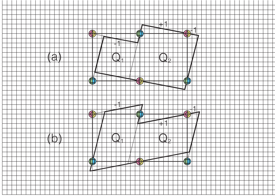
FIGURE 2. Partition of the torus
